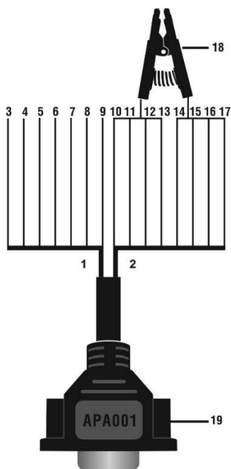
Figure 2-5 EEPROM Clamp Integrated MC9S12 Cable
